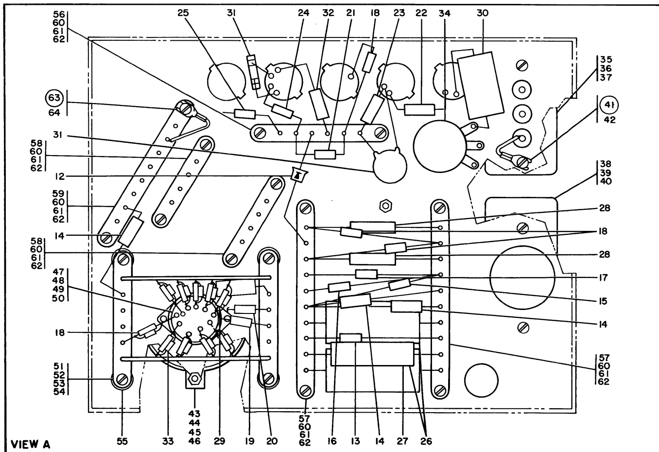
FIGURE 12. CHASSIS ASSEMBLY. SEE LIST 12.
